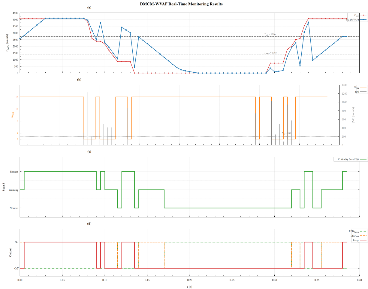
Figure 7: Visualisasi Data Hasil Simulasi DMCM-WVAF Menggunakan GNUPlot. Panel (a) ADC Raw vs WVAF Filtered; Panel (b) Window Size ( N_{win} ) dan Impuls Perubahan Absolut ( |\Delta V| ); Panel (c) Criticality Level / System State ( S_k ); Panel (d) Sinyal Kontrol Aktuator digital (Green LED, Red LED, Relay).
